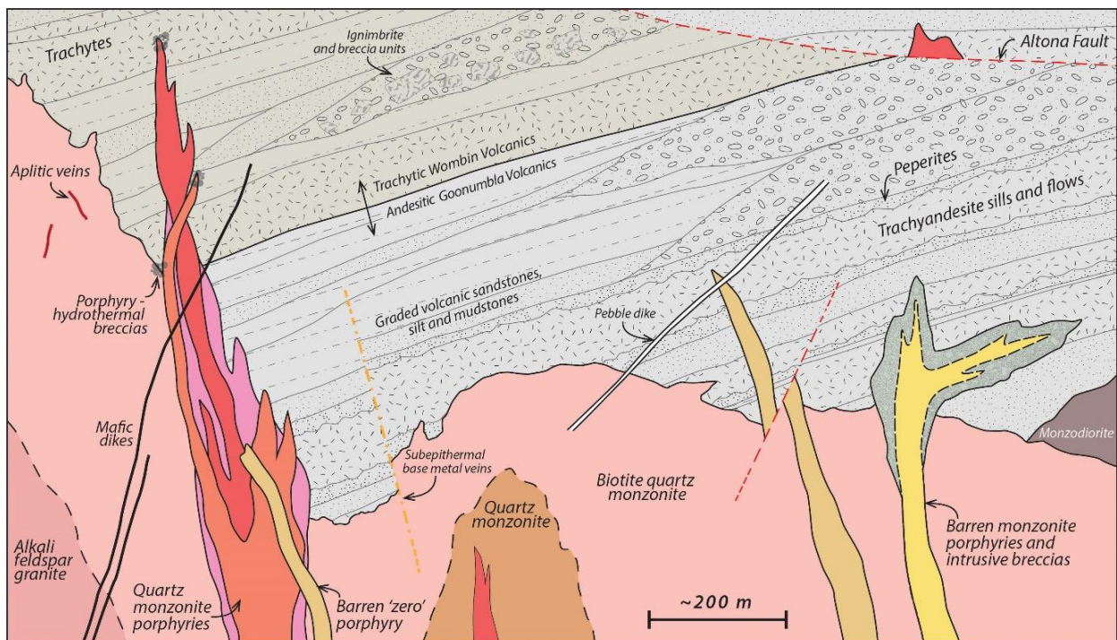
Figure 1: Schematic depiction of the mineralisation and major rock types encountered at Northparkes)
